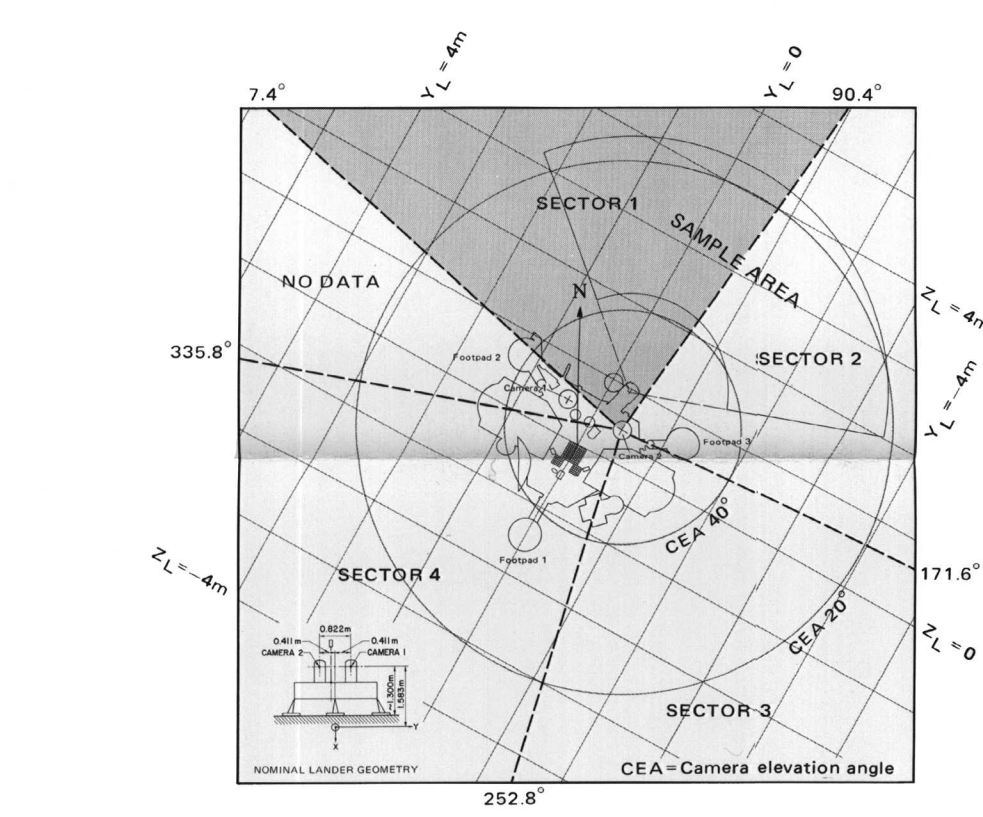
7.4° 90.4° 336.8° 171.6° 202.8° VERTICAL VIEW SHOWING VIKING LANDER 2 ORIENTATION Grid is in spacecraft coordinates
